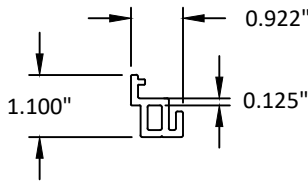
9 BOTTOM RAIL REINFORCEMENT
