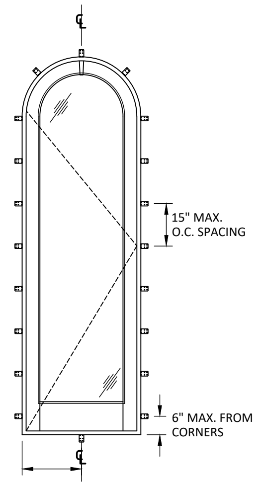
ANCHOR LAYOUT INSTALLATION CLIP
