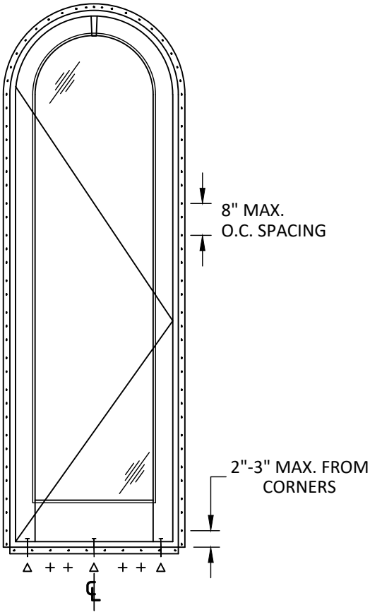
ANCHOR LAYOUT NAIL FIN
