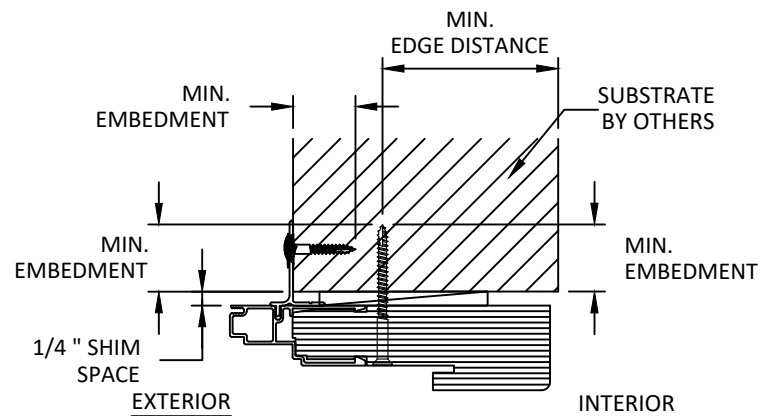
A 12 ANCHOR DETAIL NAIL FIN (HEAD)
